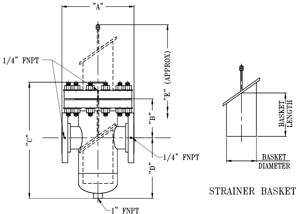
STRAINER HOUSING
