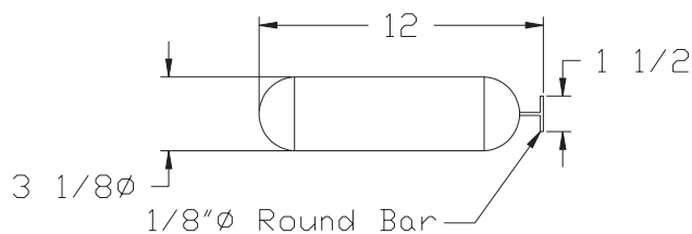
DISPLACEMENT BALLOON
